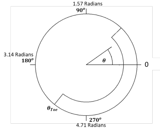
Figure 7—Morrell charge co-ordinate system (after Morrell, 1993)
